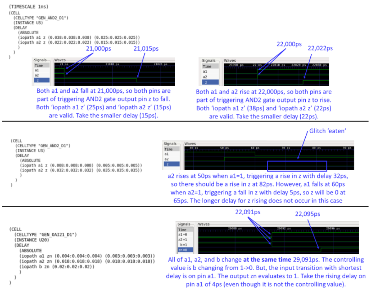
Figure 3. Additional clarifications regarding SDF file interpretation.
