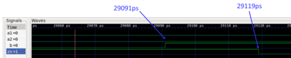
Figure 2. Example interpretation of SDF file and glitch enabled simulation results.
